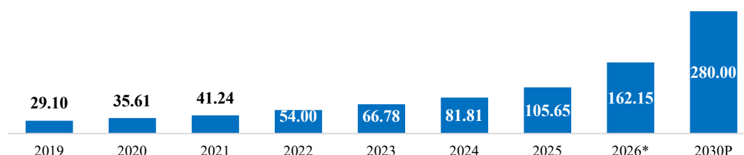
Solar Energy Capacity in India (GW) (Years in FY)
